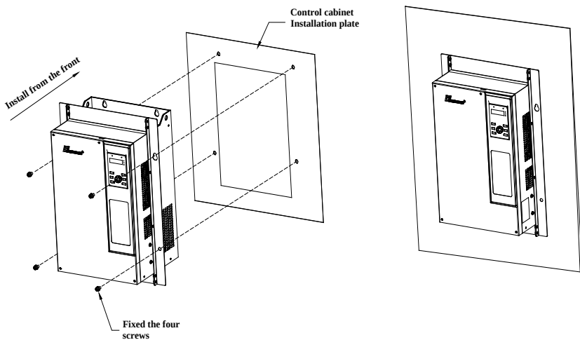
Diagram2-9 Sheet metal structure embedded mounting diagram
