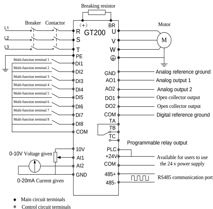
Diagram2-19 Diagram of wiring for basic running
