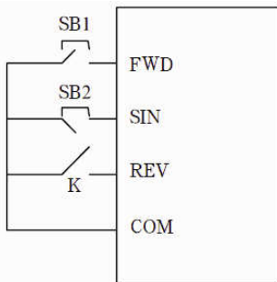
Illustration: 3-wire control model 2
