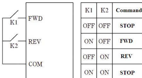
Illustration: 2-wire control model 1
